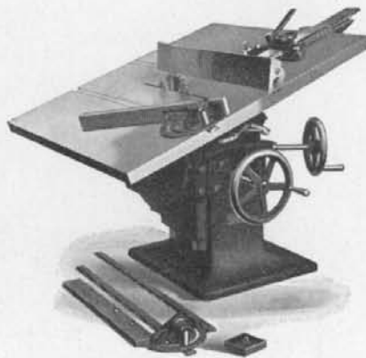
No. 493 Tilting-Table Saw Motor on Arbor or for Belt Drive
