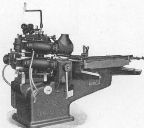
No. 533 Single End Tenoner With Built-in Motors
