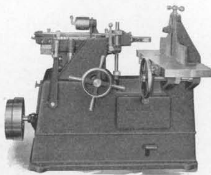
No. 214 Horizontal Mortiser Chisel Capacity up to 1\frac{1}{2} "
