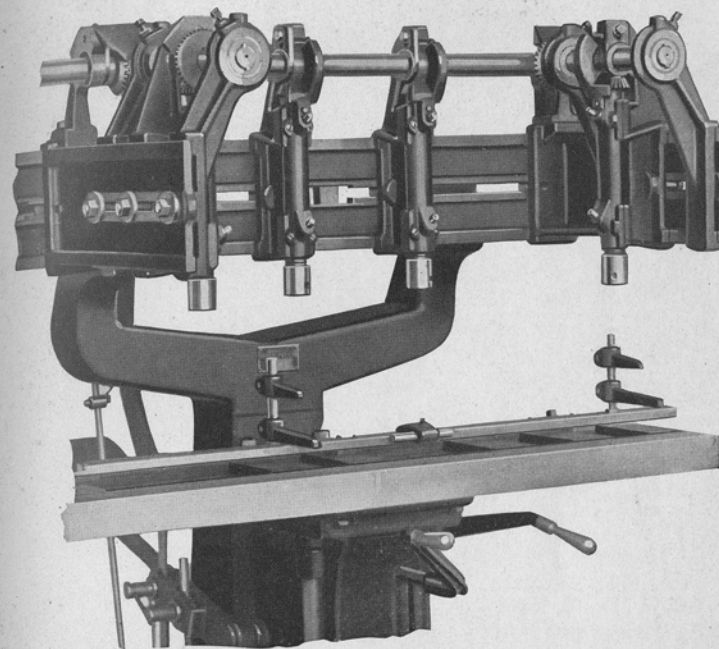
Extension Brackets and No. S-2 Heads on No. 369 Borer
