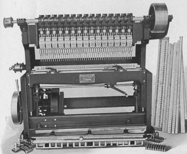
No. 375 Piano Player Part Gang Borer
