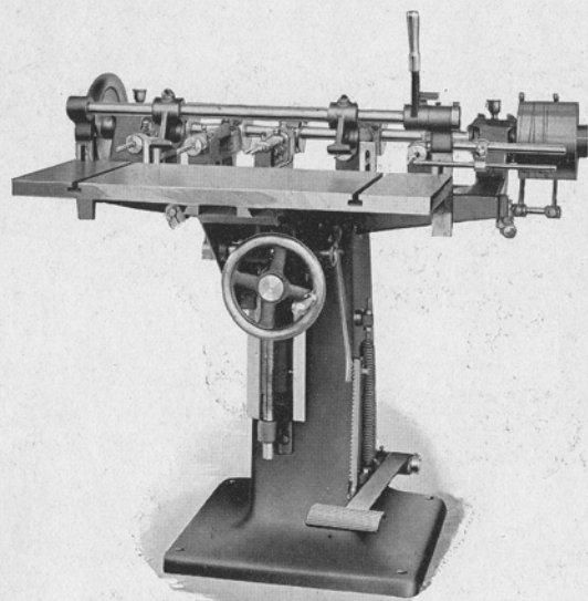
No. 368 Pedestal Column Horizontal Gang Borers
