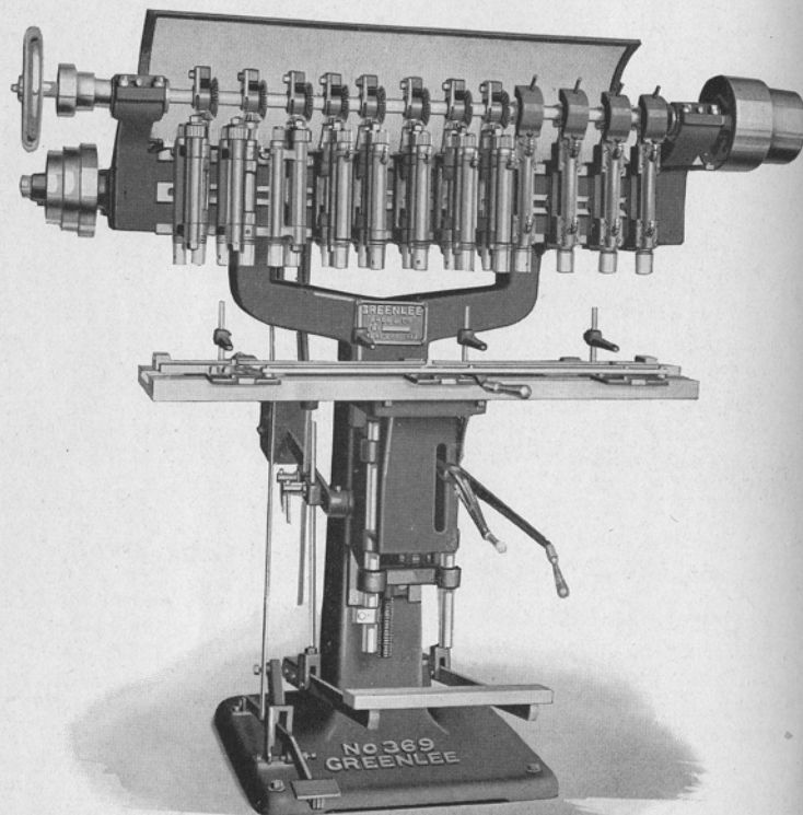
No. 369 4-ft. Borer with Power Feed
