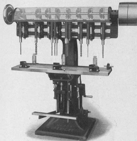
No. 369 3-ft. Borer with Foot Feed
