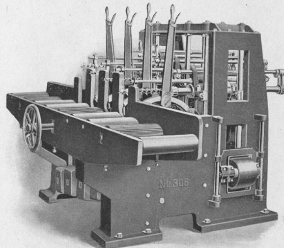
No. 306 Extra Heavy Four Spindle Car Borer
