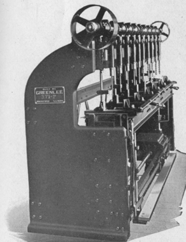
No. 371 with Screw Power Feed
