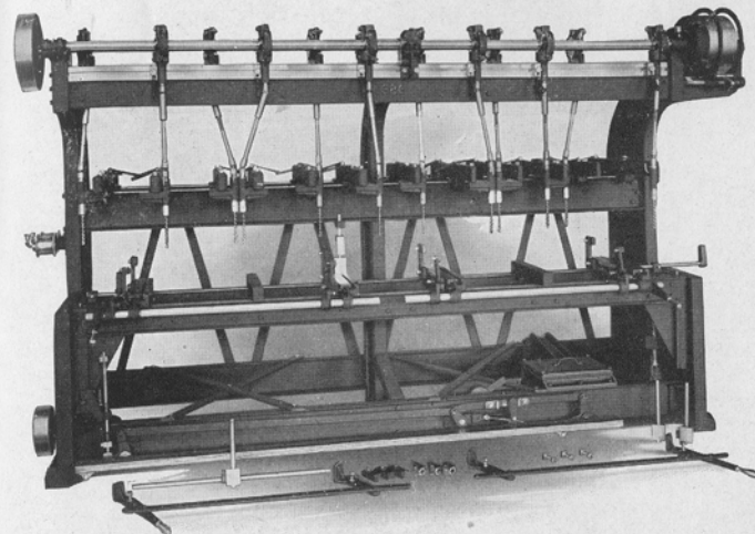
No. 386 10-ft. Borer with Screw Power Feed
