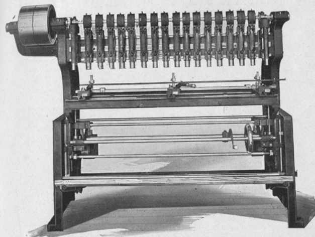
No. 371 with Foot Feed
