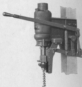
No. 357-A Post Borer
