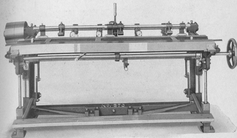
No. 370 Double Column Horizontal Gang Borers
