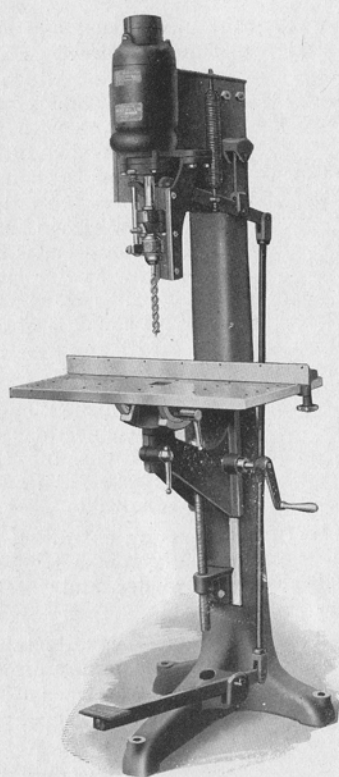
No. 357 Light Pattern Borer with Built-in Motor
