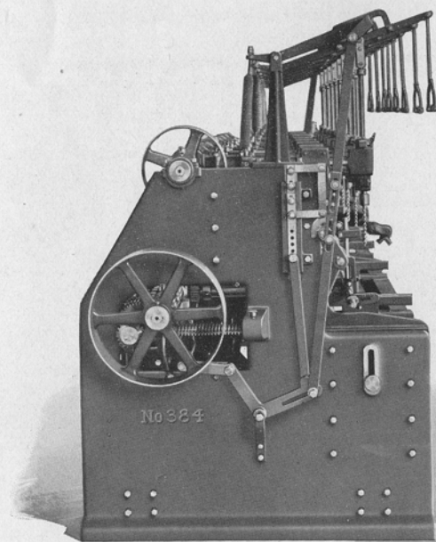
End View of No. 384 with Power Clamp
