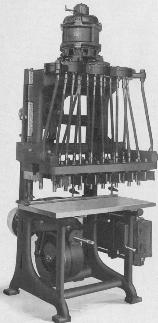
No. 364 Universal Spindle Vertical Gang Borer
