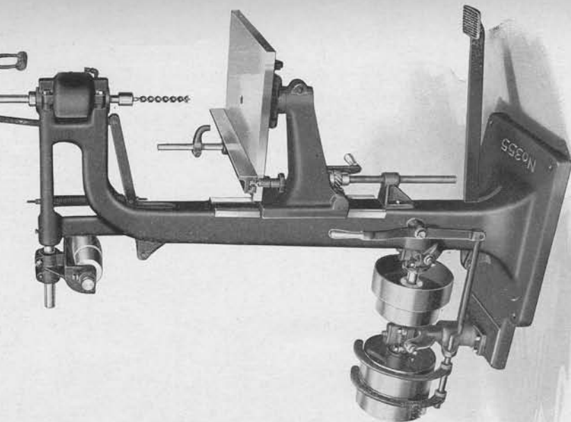
No. 355 Single Spindle Vertical Borer
