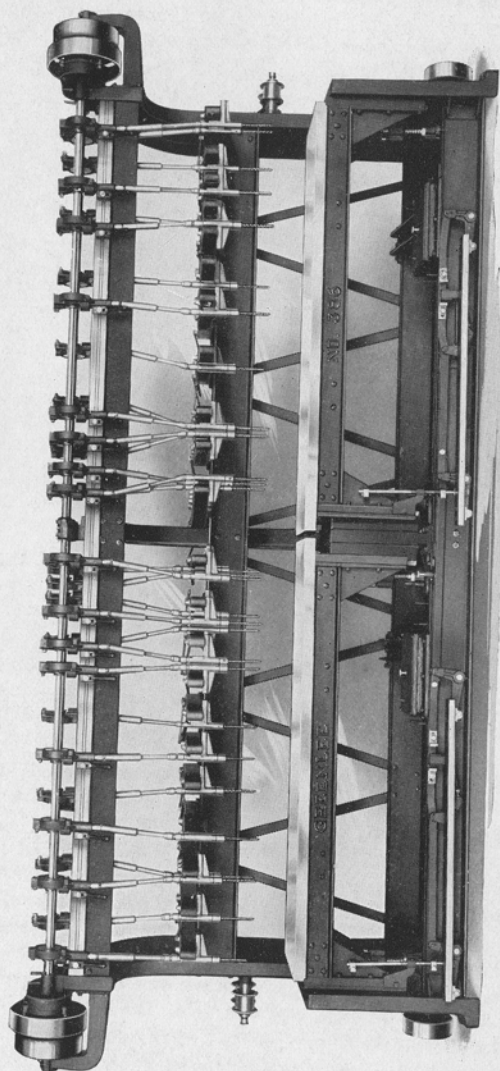
No. 386 14-ft. Universal Spindle Gang Borer With Screw Feed Tables
