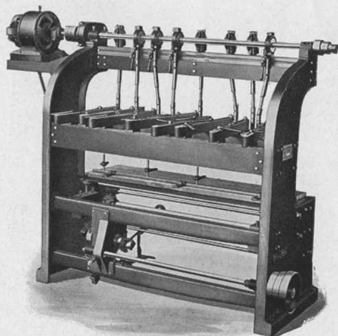
Rear View of 6-ft. No. 386 with Motor
