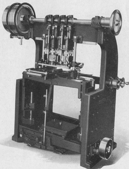
No. 374 Extra Range Double Column Gang Borer
