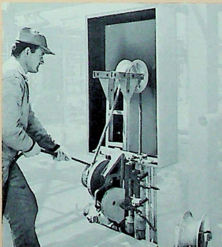
Setup for "up" pull. 640 power puller mounted on 649 pipe adapter sheave, which is clamped to 4" service conduit coming from slab. Complete system setup time: less than two minutes.
