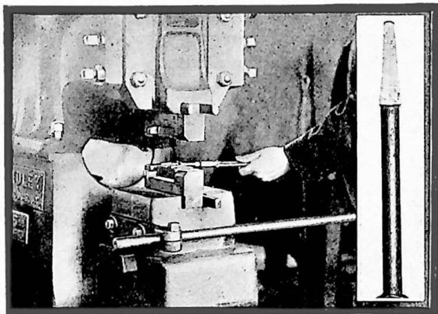
Forming the Square
