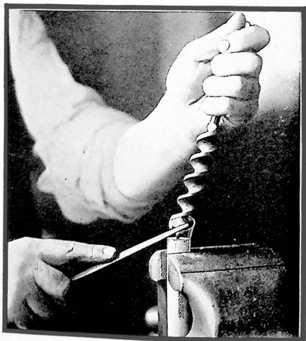
Filing the Bottom of Cutting Edges
