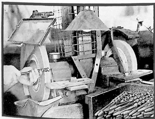
Grinding Clearance Back of Head
