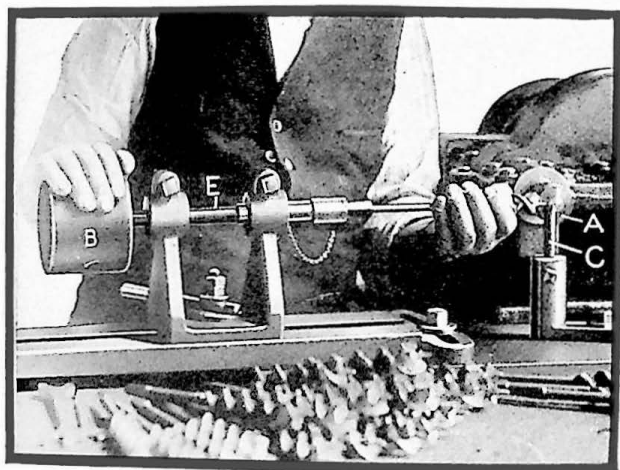
Threading the Point
