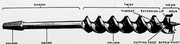
The Parts of an Auger Bit
