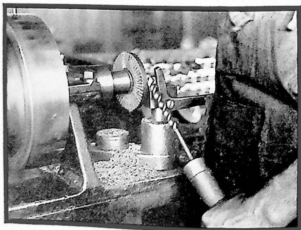
"Facing" or Squaring Up Cutting Edges
