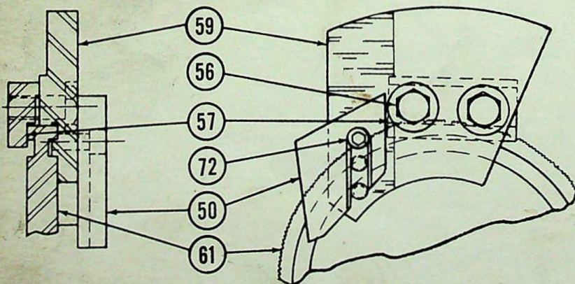
RETURN CAM PLATE 3RD POS.
