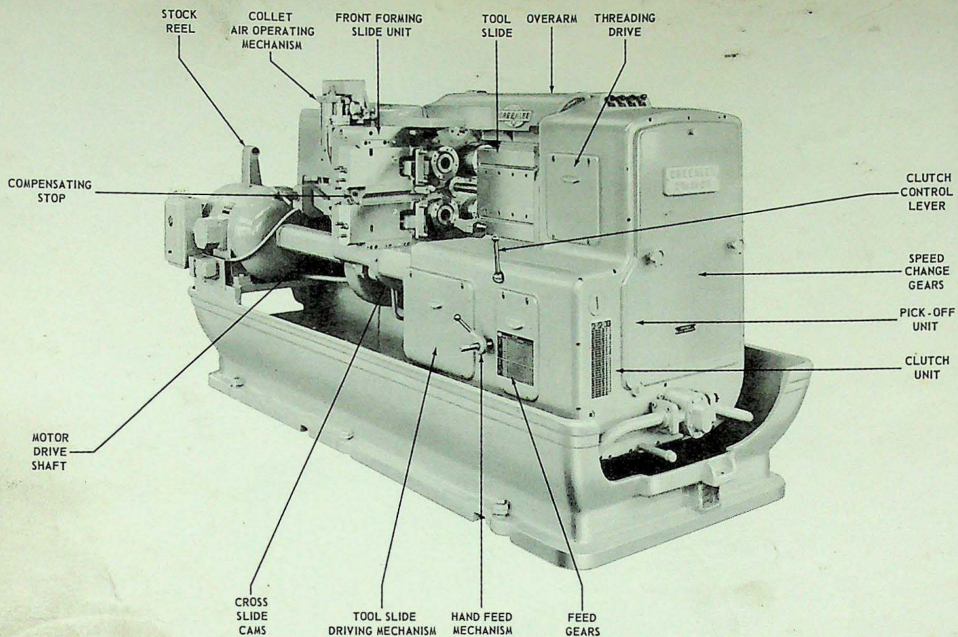
FRONT VIEW
