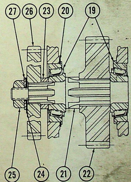
DETAIL "F"
