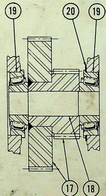
DETAIL "B"
