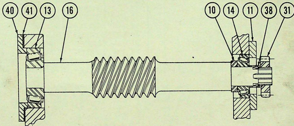
DETAIL "D"
