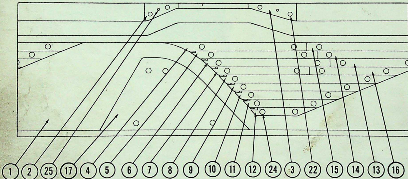
Developed view of cam drums showing cam strips.
