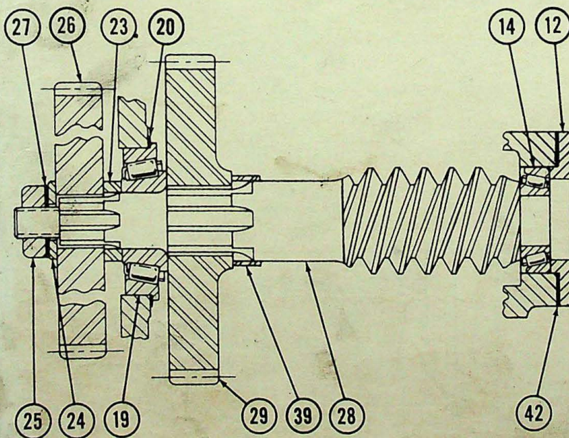
DETAIL "E"
