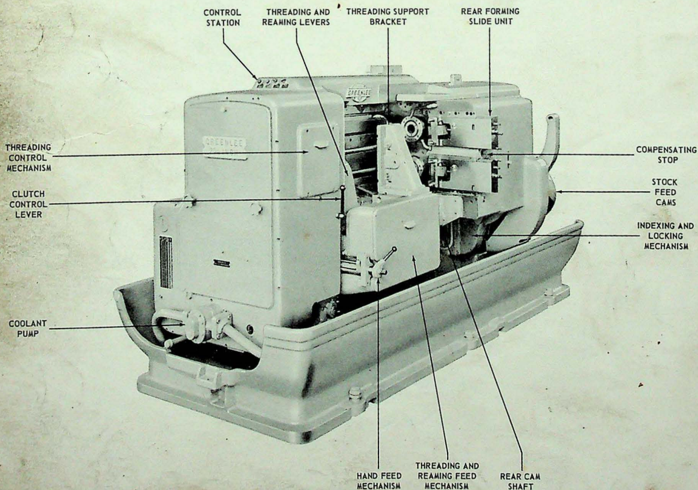
REAR VIEW
