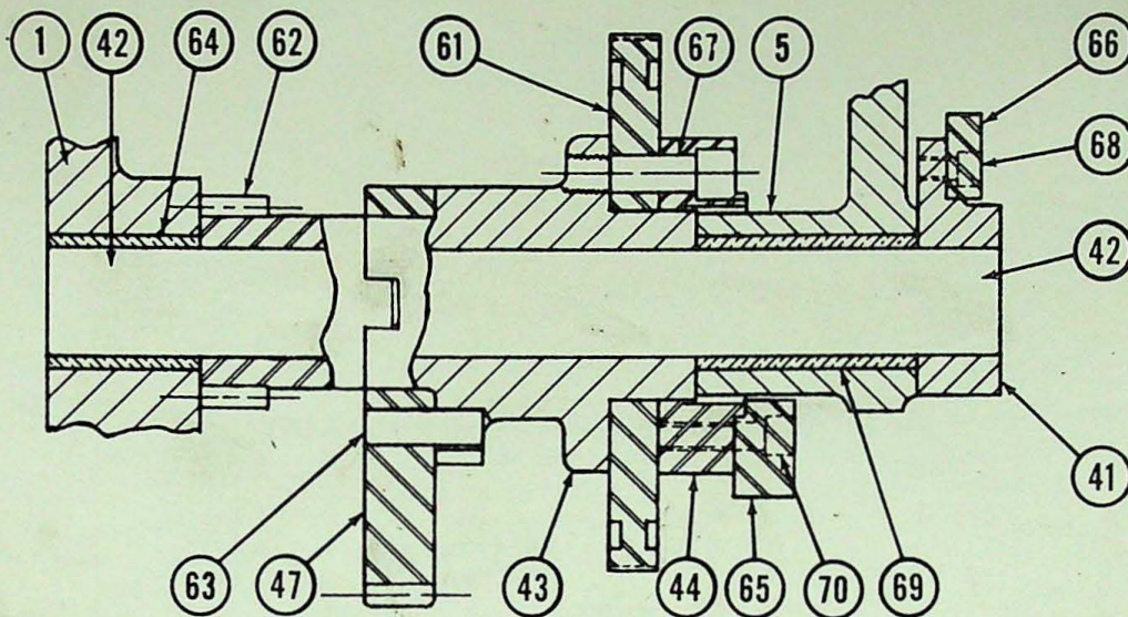
DETAIL "A"
