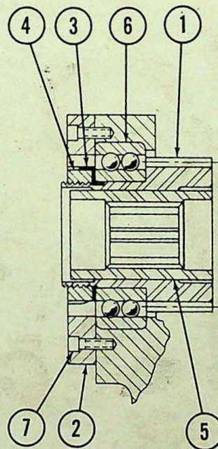
DETAIL "A"
