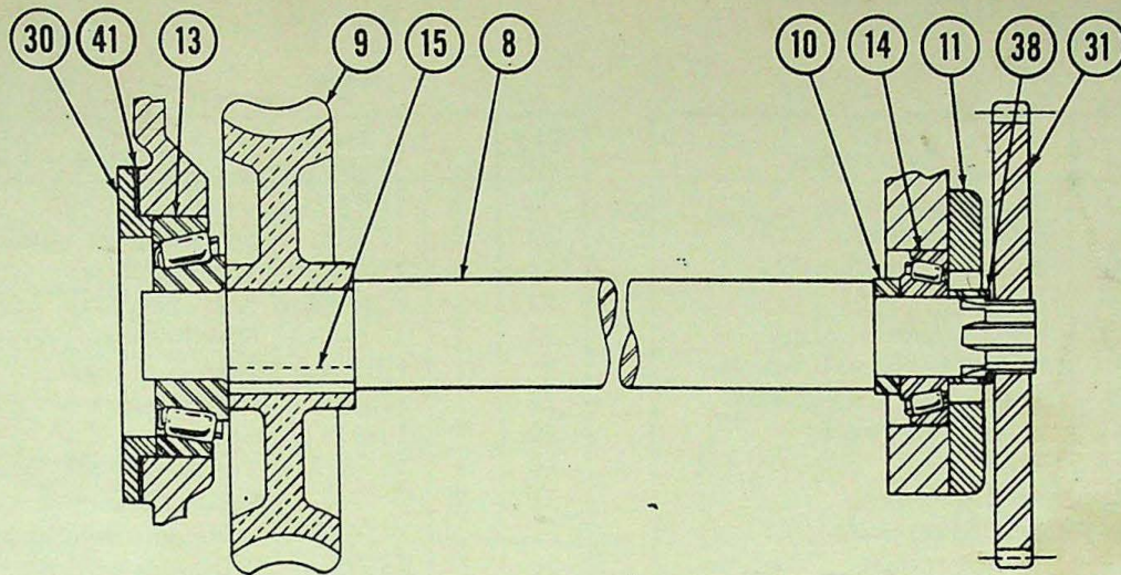
DETAIL "C"
