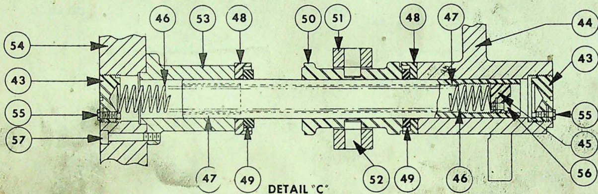
DETAIL "C"
