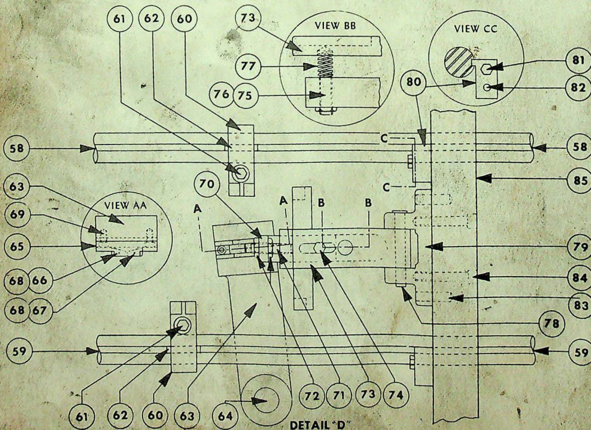
DETAIL "D"
