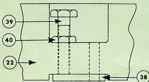
STOCK REEL LEVELING PLATE DETAIL
