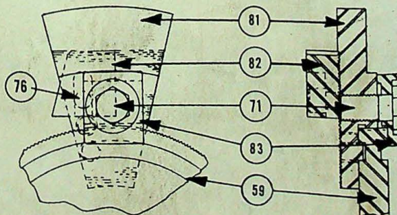
FEED CAM PLATE 5TH & 6TH POS.
