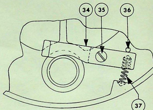
STOCK REEL LOCKING FINGER DETAIL
