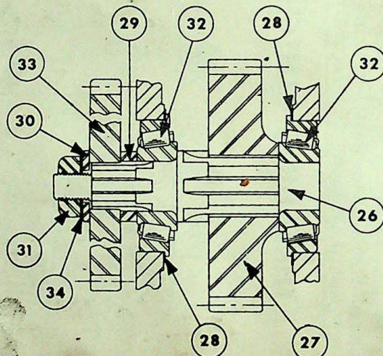
DETAIL 'E'
