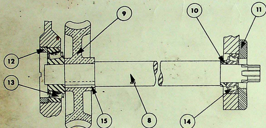
DETAIL 'B'
