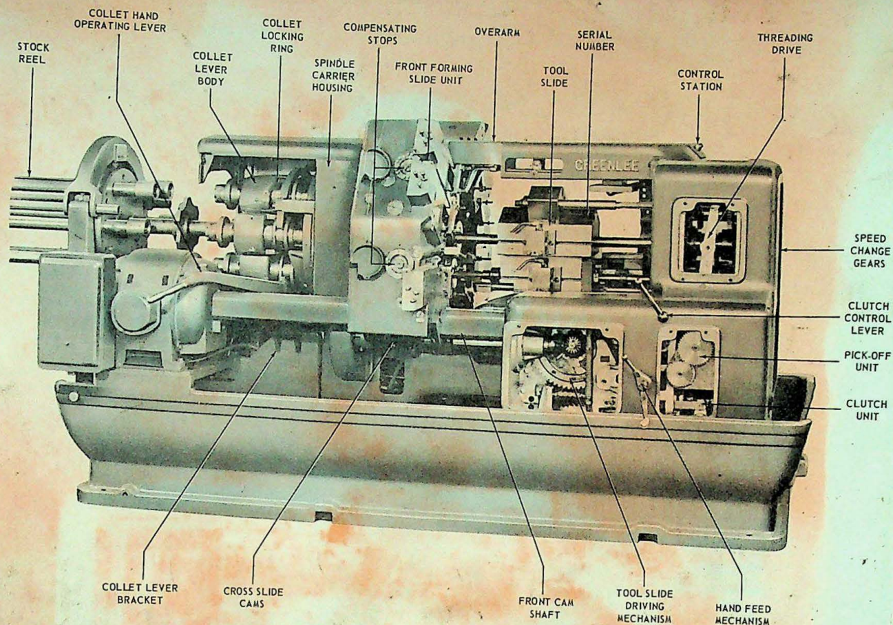
FRONT VIEW
