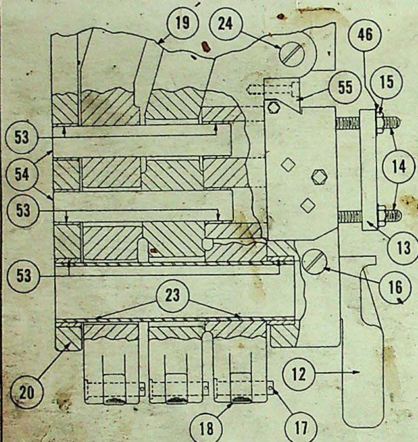
Front Forming Slide Unit
