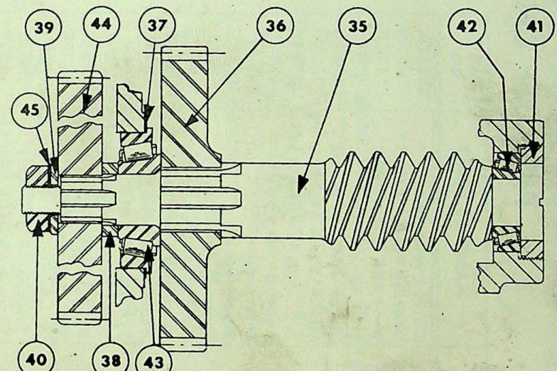
DETAIL 'F'
