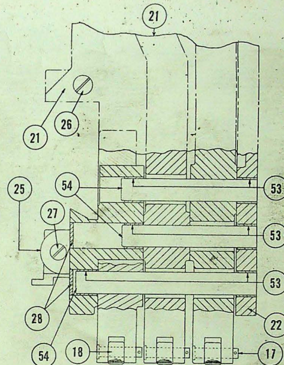
Rear Forming Slide Unit
