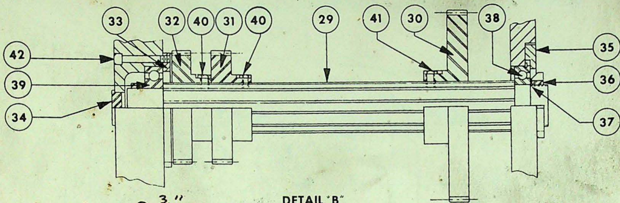
DETAIL "B"
