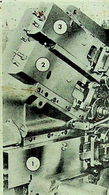
Front Forming Slide Unit
