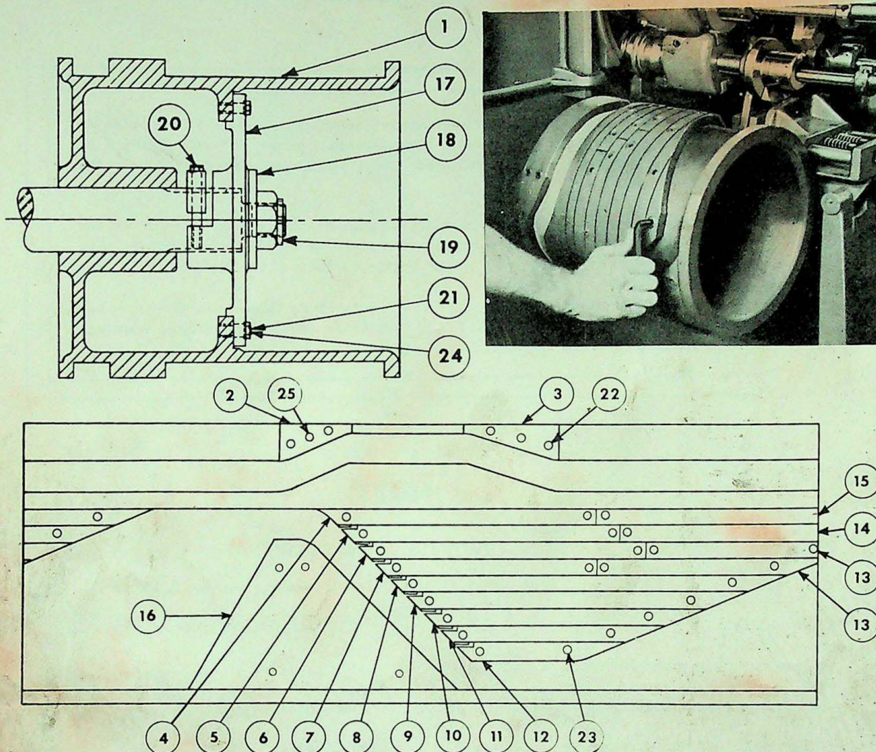
DEVELOPED VIEW OF CAM DRUM SHOWING CAM STRIPS
