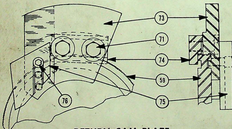
RETURN CAM PLATE 3RD & 4TH POS.
