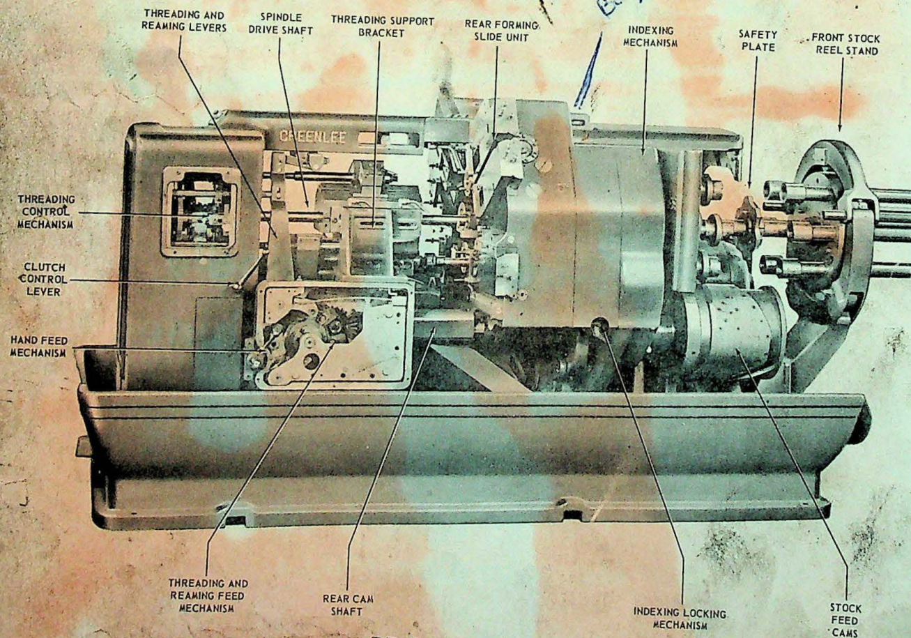
REAR VIEW
